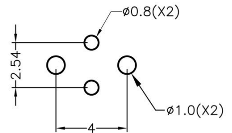
MOUNTING HOLES
